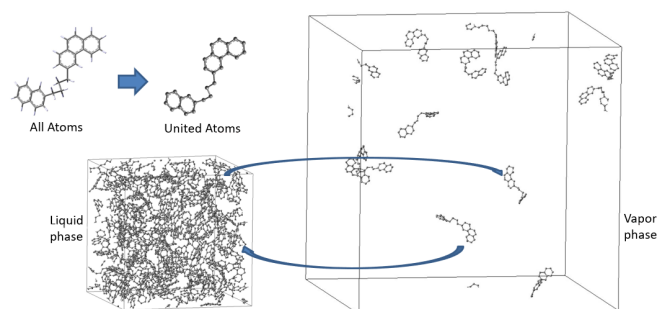
Figure 1: Schematic view of vapor-liquid equilibrium simulation of a polyaromatic hydrocarbons using the extended TraPPE-UA forcefield for polycyclic flexible molecules 5 .
