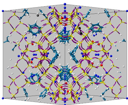
Figure 2: Example configuration of adsorption of a multicomponent gas mixture in NaY faujasite.
